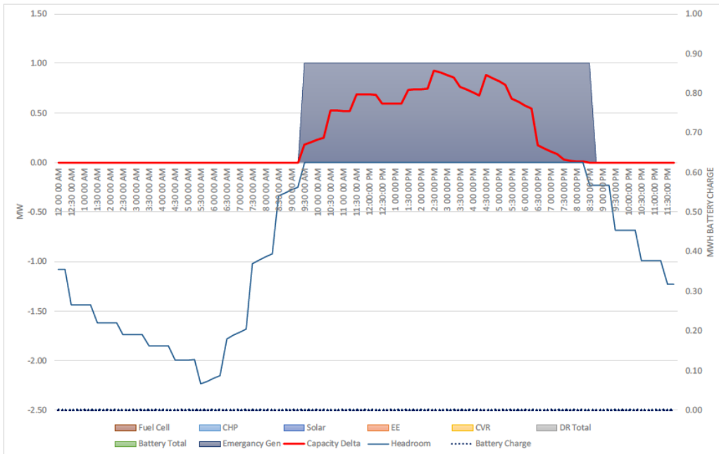
Figure 24: 31W1 2029 peak day dispatch model for mobile generation
