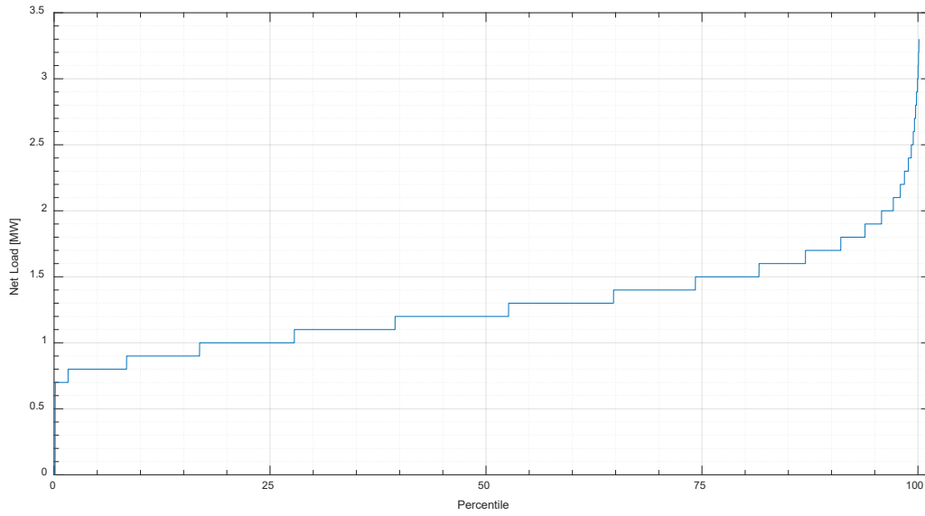
Figure 39: 2019 Load Percentiles Net Load Data at 31W2
