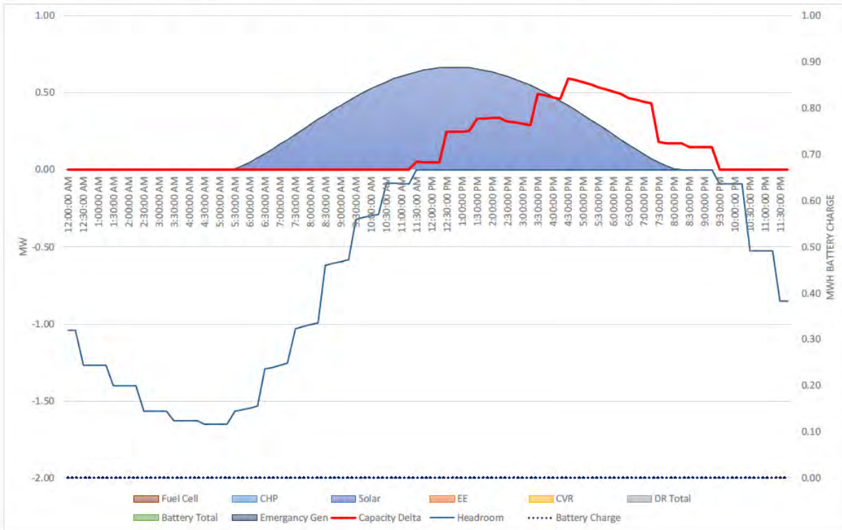
Figure 23: Weather Adjusted Solar Capacity Offsetting Capacity Need at 31W2
