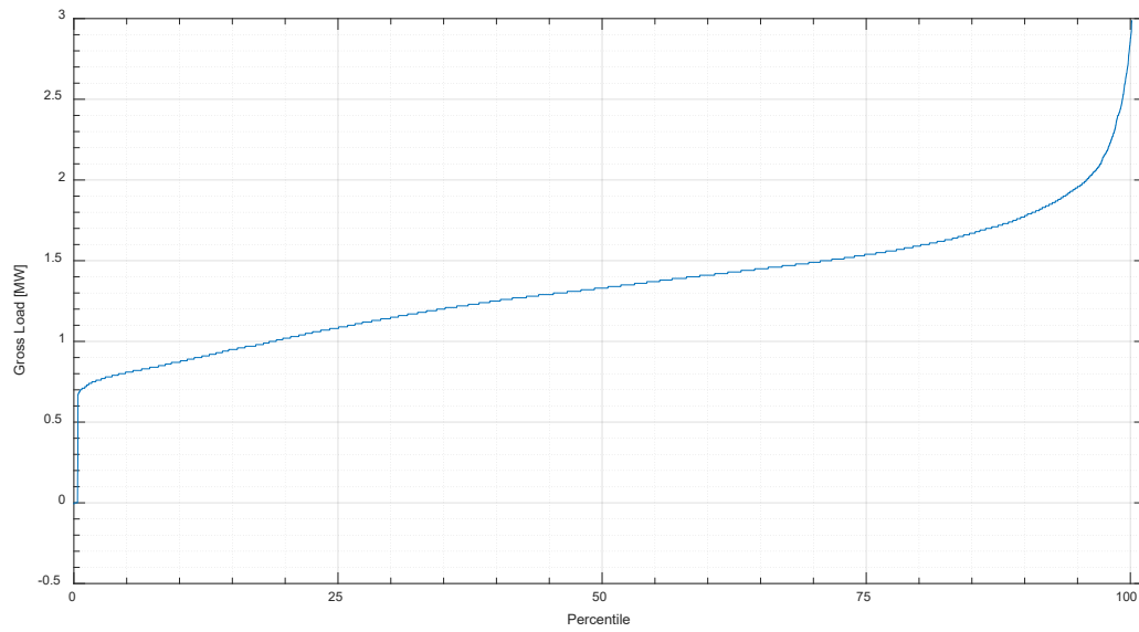
Figure 41: 2019 Load Percentile Gross Load Data at 31W2
