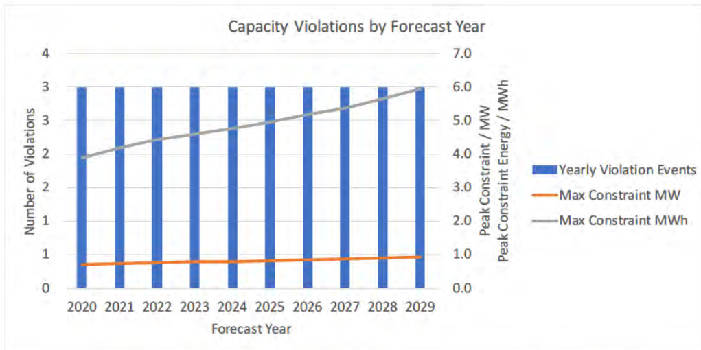
Figure 11: Capacity Violation Characteristics for 31W1 by Forecast Year from the NWA Screening Tool
