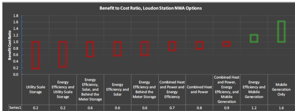
Figure 1: Benefit to Cost Ratio of Loudon Station NWA Options
