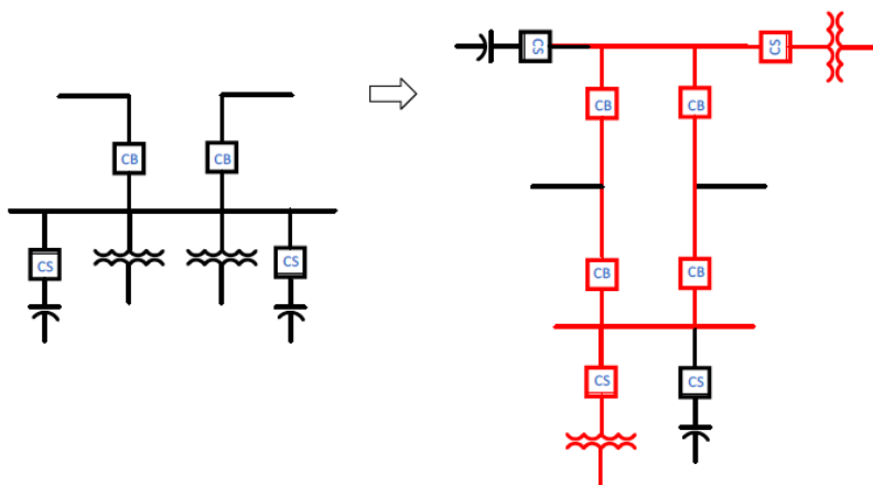
Figure 1: Modification for White Lake Substation Design
