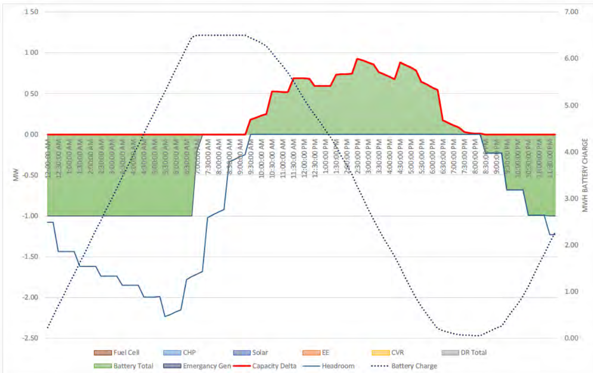
Figure 20: Battery Dispatch Model 31W1 during 2029 peak day
