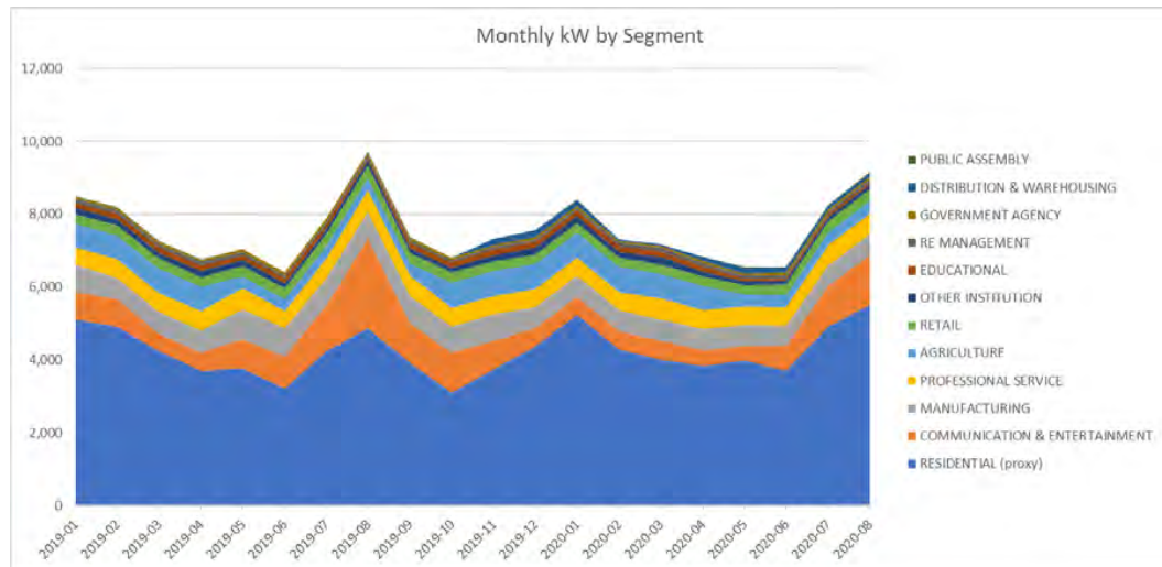
595 Figure 37: Monthly kW Load by Rate Class
