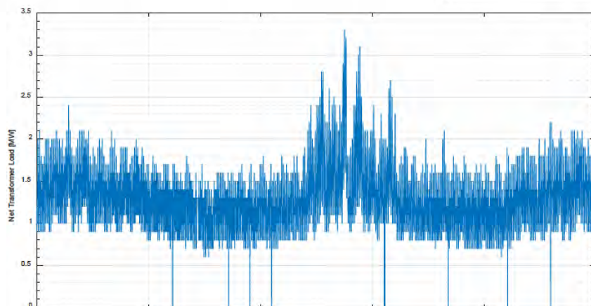
Figure 12: 2019 Time Series Net Load Data at 31W2 Loudon Station
