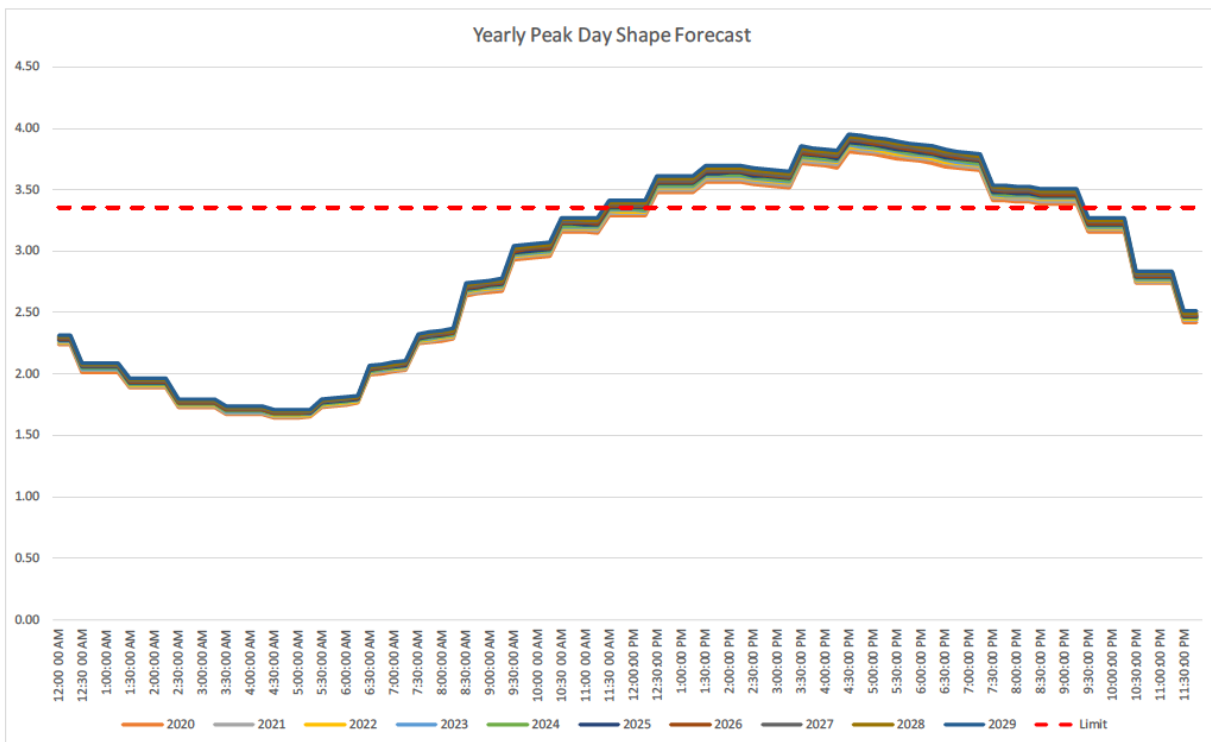
Figure 13: Forecasted Net Load Shapes for Peak Day by Year at 31W2 from the NWA Screening Tool
