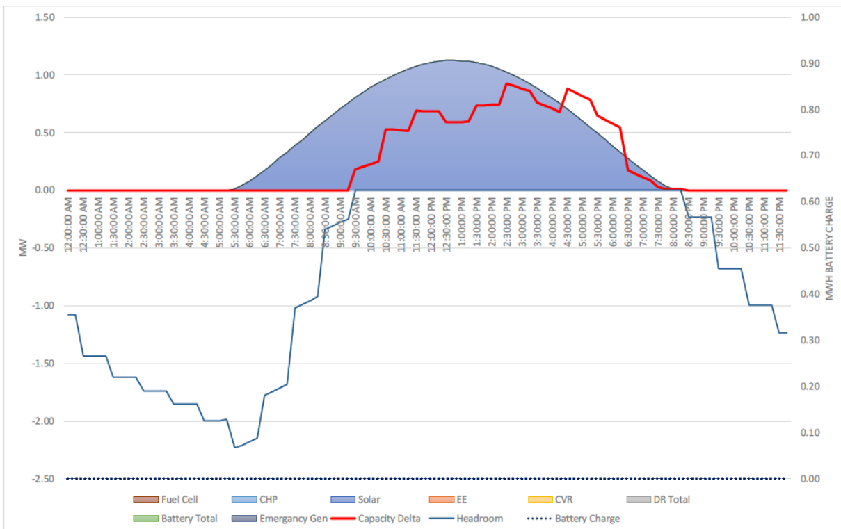
Figure 22: Weather Adjusted Solar Capacity Offsetting Capacity Need at 31W1
