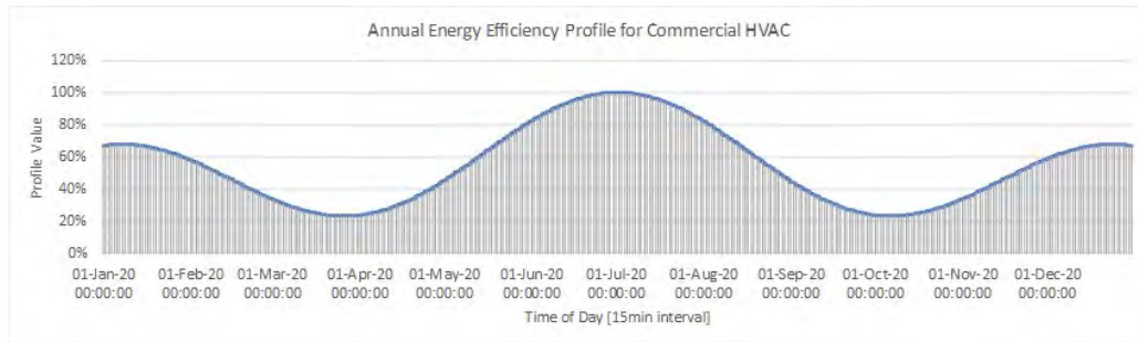
324 Figure 4: Annual Commercial HVAC EE Profile
