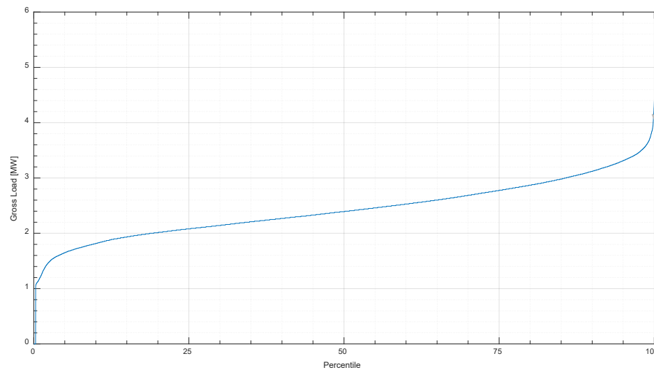
Figure 8: 2019 Load Percentile Gross Load Data at 31W1
