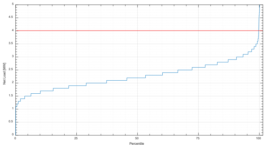
Figure 6: 2019 Load Percentiles Net Load Data at 31W1
