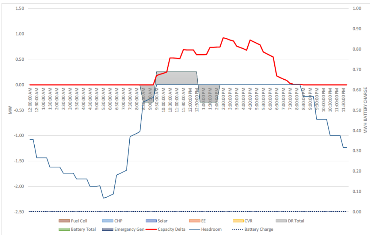
280 Figure 19: Three-hour demand response event at 31W1 with preconditioning and snap back
