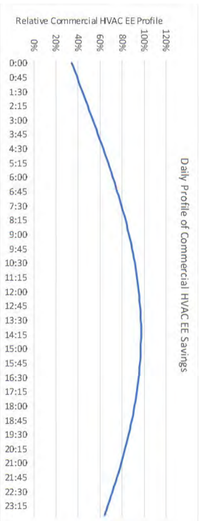
Figure 5: Daily Profile for Commercial HVAC EE
