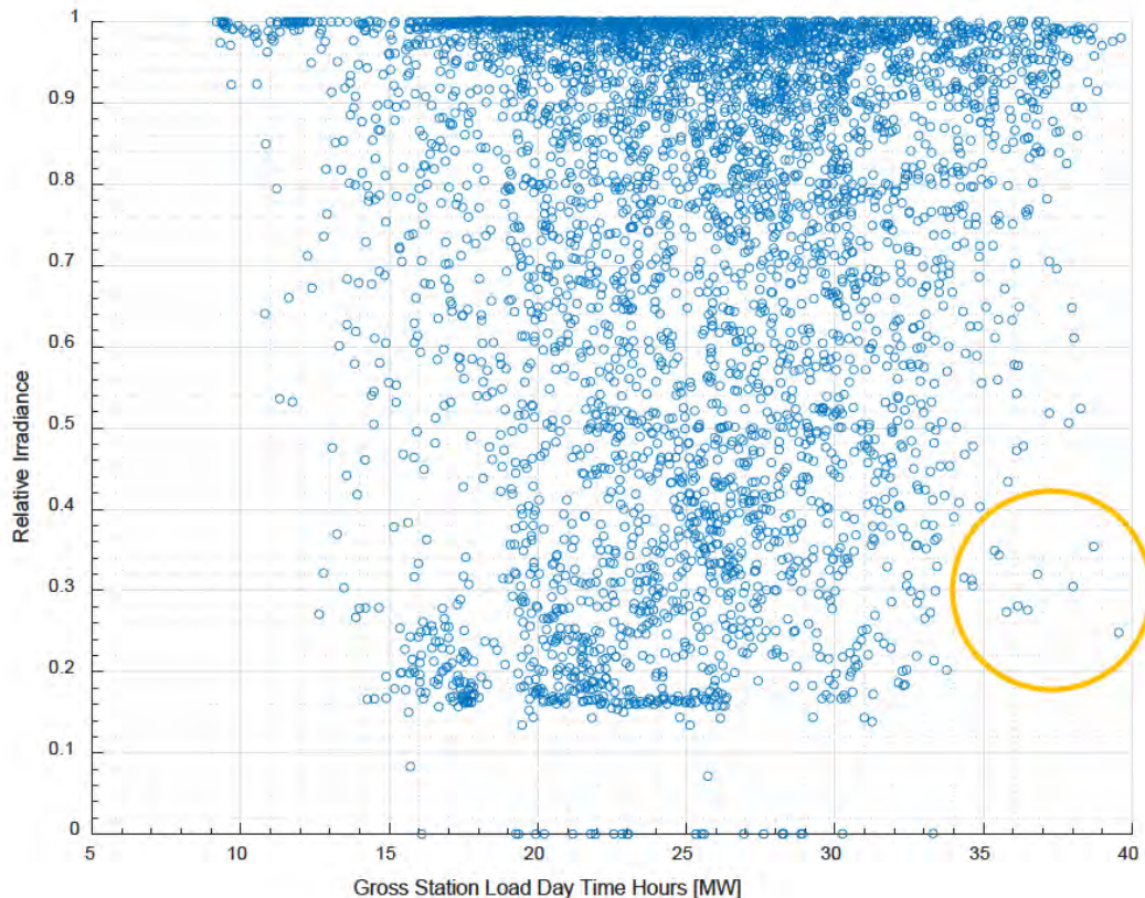
577 Figure 32: Sample Station Relative Irradiance Profile over Station Load
