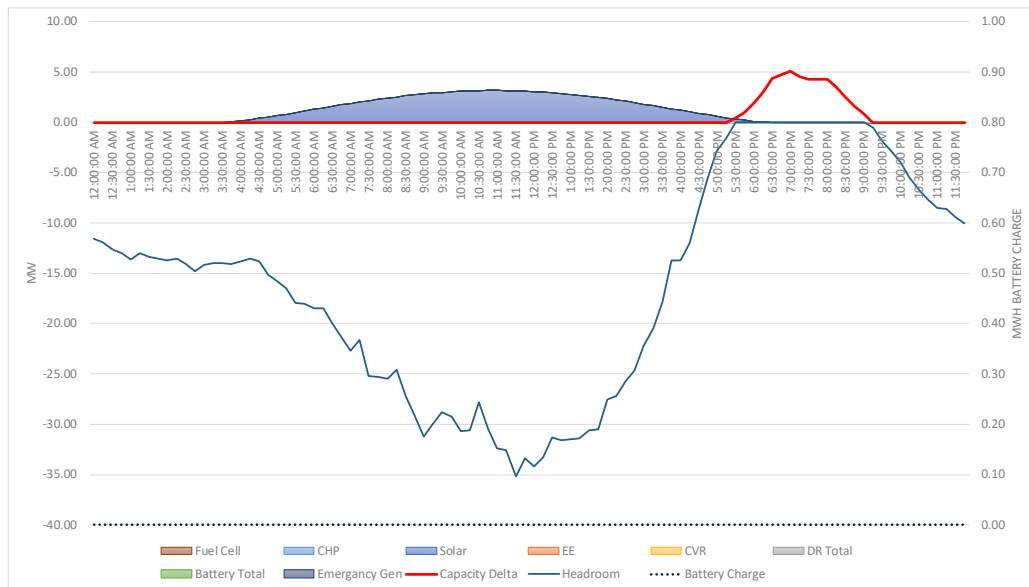
298 299 Figure 2: Application of Minimal Weather Adjusted Solar Generation Capacity to a Capacity Deficit
