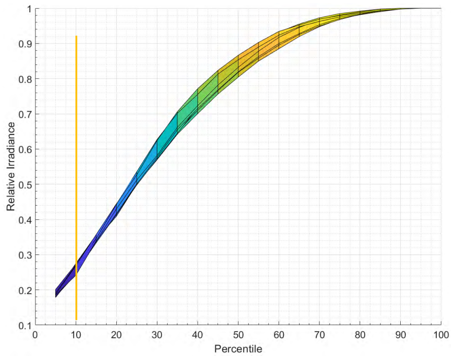
Figure 34: 10th Percentile Relative Irradiance
