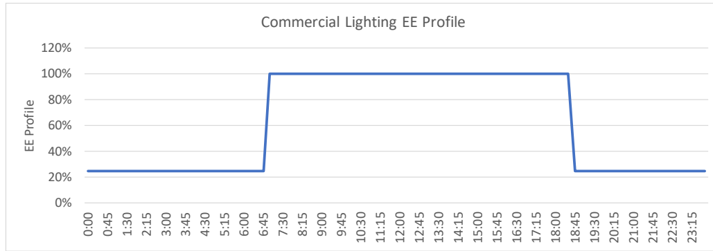
312 Figure 3: Daily Lighting EE Profile
