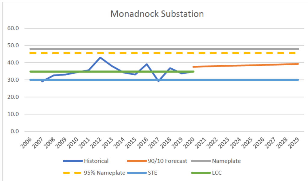
Figure 3. Monadnock capacity and historical and forecasted load
