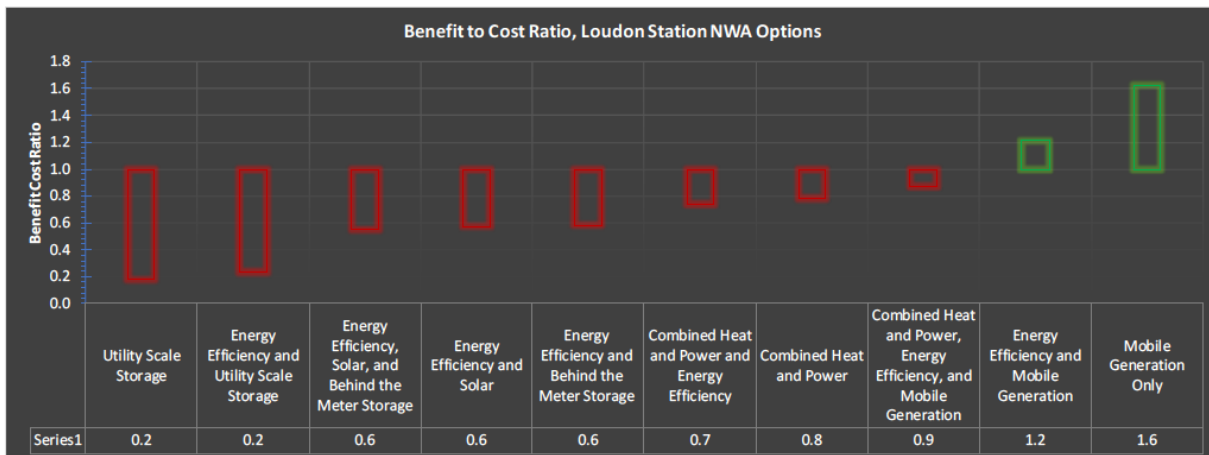
531 Figure 29: Benefit to Cost Ratio of Loudon Station NWA Options
