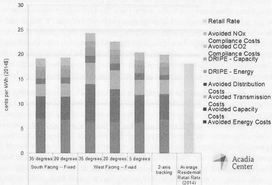
Figure 1: Grid Value of Solar PV in NH – 25-year Levelized Cost (2014$)
