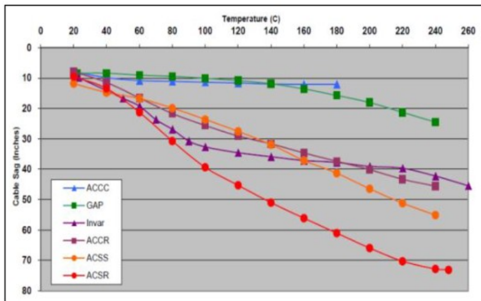
Figure 2 - Sag / temperature comparison of several conductors tested by Ontario Hydro at Kinectrics lab. The graph not only shows the substantially reduced sag, it also shows the particular ACCC ® conductor tested operated at 60° to 80° C cooler than the other conductors tested under an equal 1,600 amp load conditions. (The conductors are listed in the sequence in which they appear from top to bottom)
