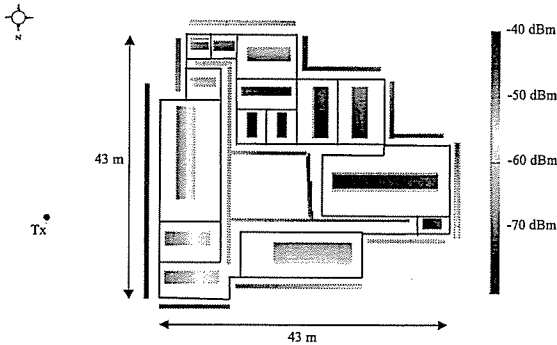
Fig. 1. RSS Layout on ground floor and street level f building A
