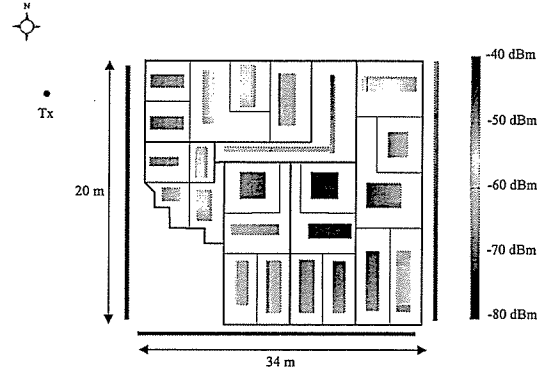
Fig. 2. RSS Layout on ground floor and street level f building C
