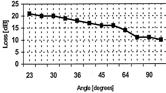
Fig. 3. Mean penetration loss against angle of incidence for the four buildings
