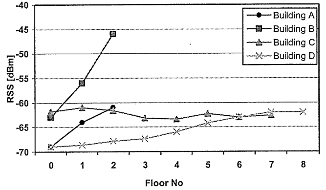
Fig. 4. Mean RSS for all floors of the four buildings
